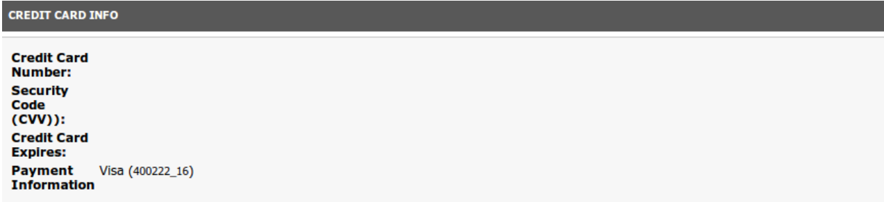
Figure 8.1: Transaction Information
