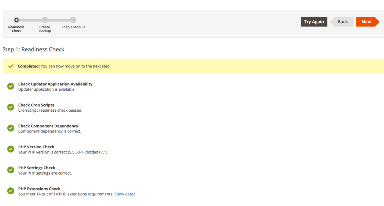
Image 8.1: Readiness Check
